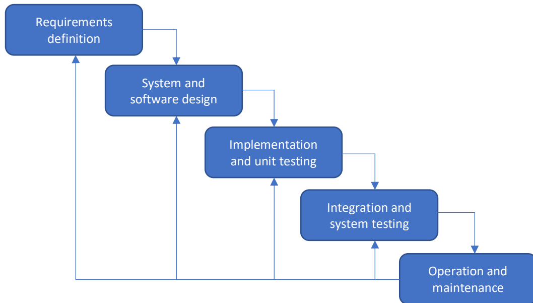
Waterfall process model
